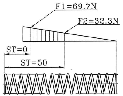
Spring force
